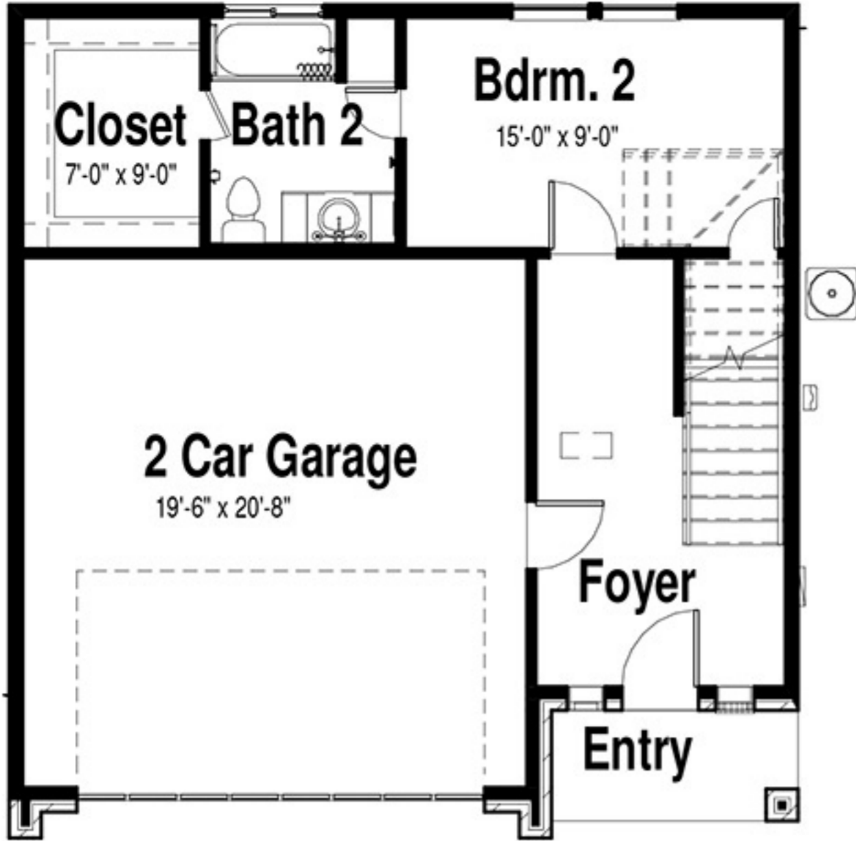
1 FIRST FLOOR PLAN - Brochure
